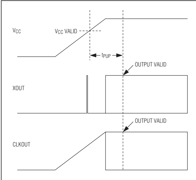
Figure 3. Power-Up Timing
