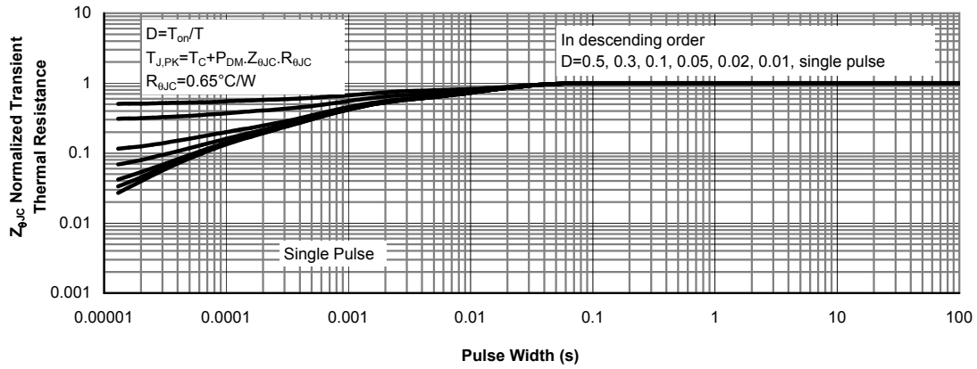
Figure 12: Normalized Maximum Transient Thermal Impedance for AOT7N60 (Note F)
