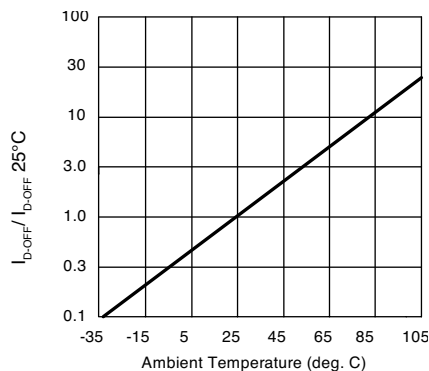
Figure 5. Typical Normalized Off-State Leakage
