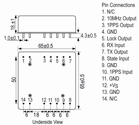
Outline (mm)
