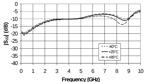
S_{22} vs. Frequency
