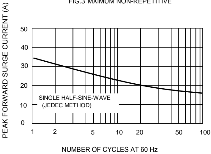
FIG.3 MAXIMUM NON-REPETITIVE
