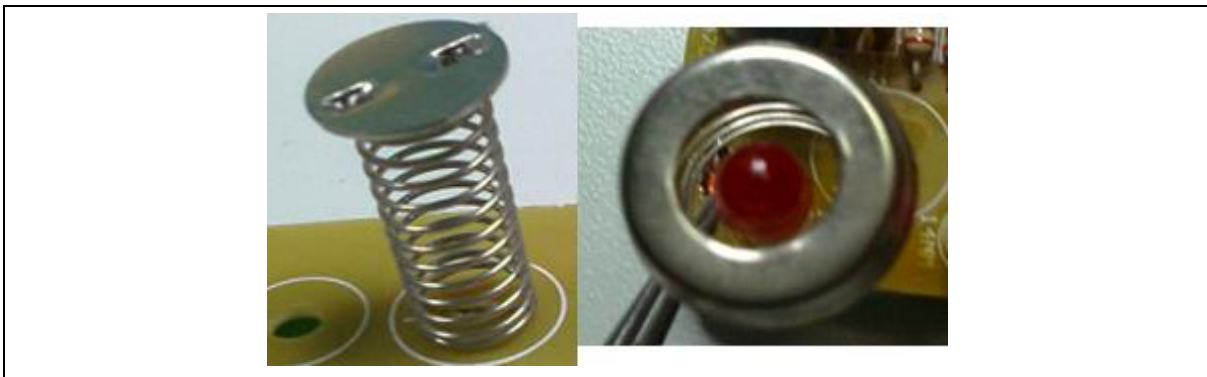
Figure 4-4 Spring with Solid Metal Plane/Ring
