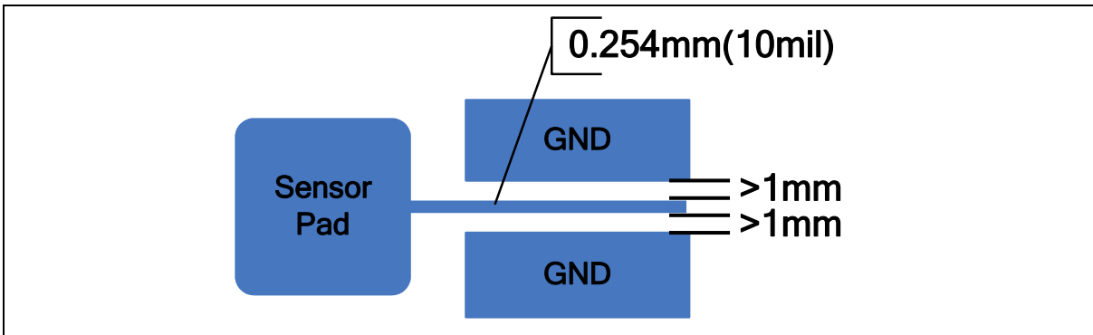
Figure 4-3 Sensor Pad and Ground-Net
