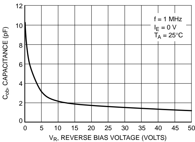
Figure 44. Output Capacitance
