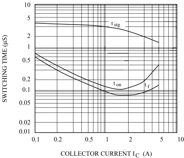
SWITCHING CHARACTERISTICS
