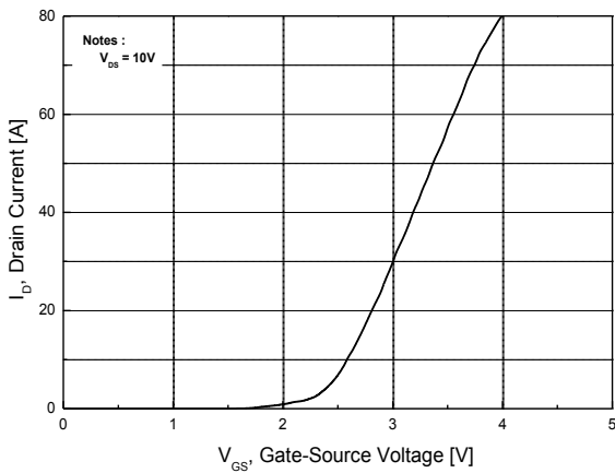
Fig.5 Transfer Characteristics
