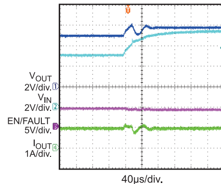
OVP Response V_{IN} from 5V to 7.5V
