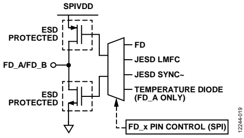
Figure 60. FD_A/FD_B Outputs
