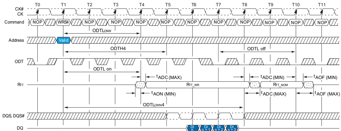
FIGURE 104 - DYNAMIC ODT: ODT PIN ASSERTED WITH WRITE COMMAND FOR 6 CLOCK CYCLES, BC4
