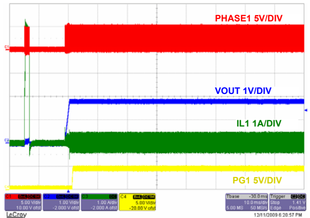
FIGURE 63. OUTPUT SHORT CIRCUIT RECOVERY (FROM HICCUP) CHANNEL 1
