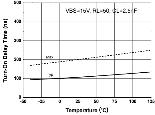
Figure 5a. Turn-On Delay Time vs Temperature
