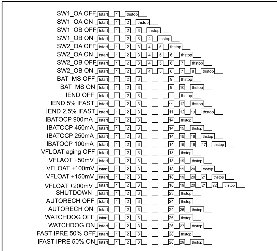
Figure 21: Single wire programming (SW_SEL INPUT)
