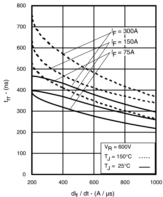
Fig 2. Typical t_{rr} vs. di/dt
