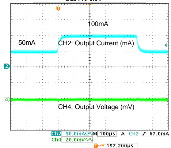
Load Transient Response BL9110-3.3V
