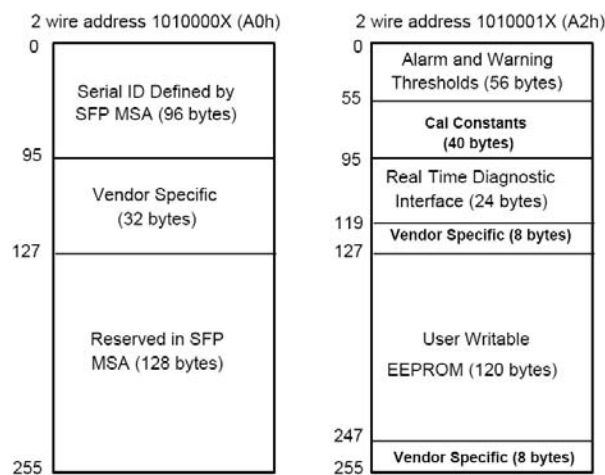
Figure 7, EEPROM Diagram
