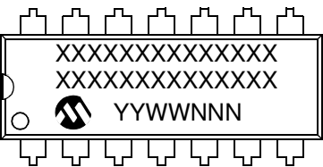
14-Lead PDIP (300 mil) (MCP6544)
