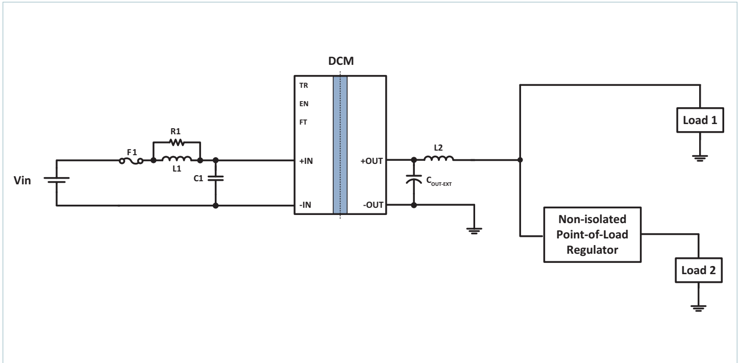
Typical Application: Single DCM3623x50M26C2y7z, to a non-isolated regulator, and direct to load
