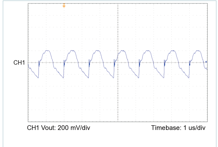
Figure 16 — Output voltage ripple, V_{IN} = 28\text{ V} , V_{OUT} = 12.0\text{ V} , C_{OUT\_EXT} = 1000\ \mu\text{F} , R_{LOAD} = 0.450\ \Omega
