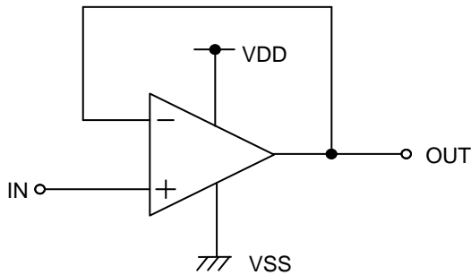
Figure 75. Voltage Follower Circuit
