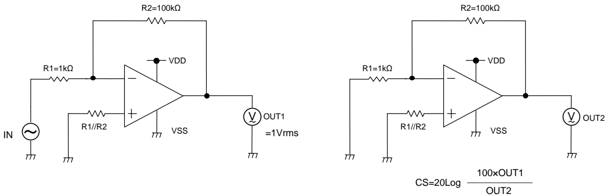
Figure 74. Test Circuit 3 (Channel Separation)
