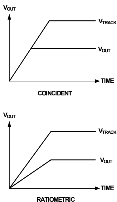
FIGURE 9. TRACKING MODES
