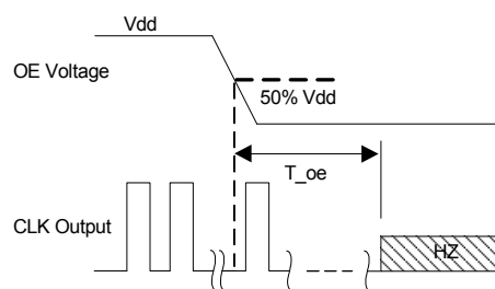
Figure 7. OE Disable Timing (OE Mode Only)
