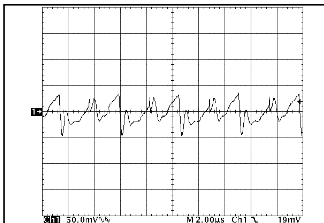
Figure 16: Output Voltage Ripple at nominal input voltage and rated load current (50 mV/div). Load capacitance: 1\ \mu\text{F} ceramic capacitor and 10\ \mu\text{F} tantalum capacitor. Bandwidth: 20 MHz. See Figure 13.
