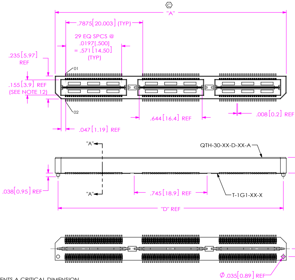
FIG 1 -A: ALIGNMENT PIN OPTION (STYLE -01 & -02 ONLY) (QTH-090-01-X-D-A SHOWN)
