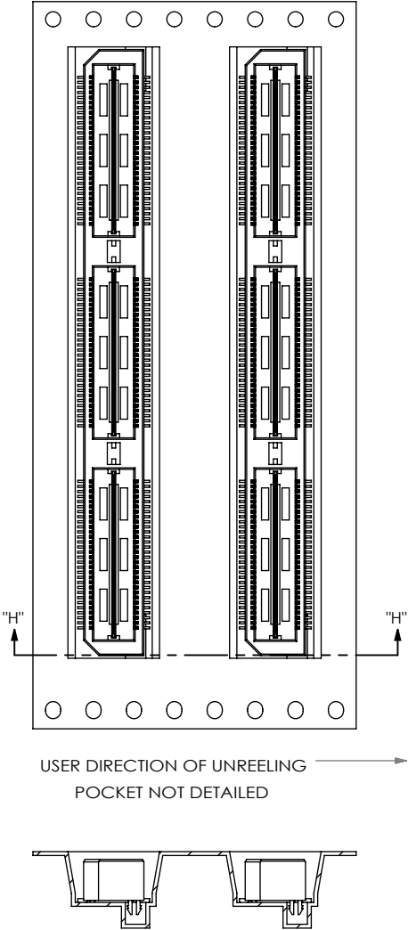
SECTION "H"- "H" SCALE 1.5 : 1
