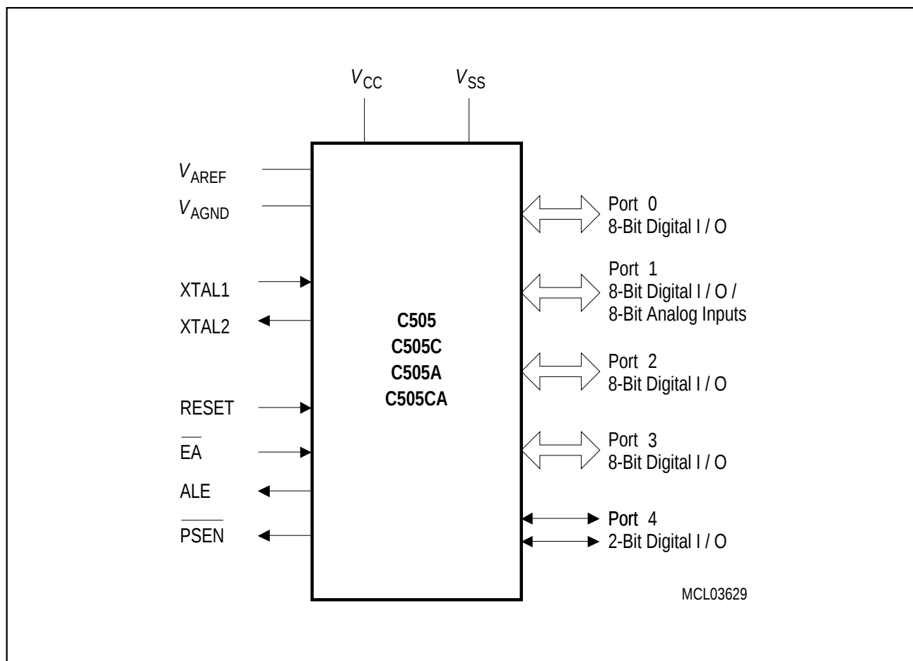
Figure 2 Logic Symbol
