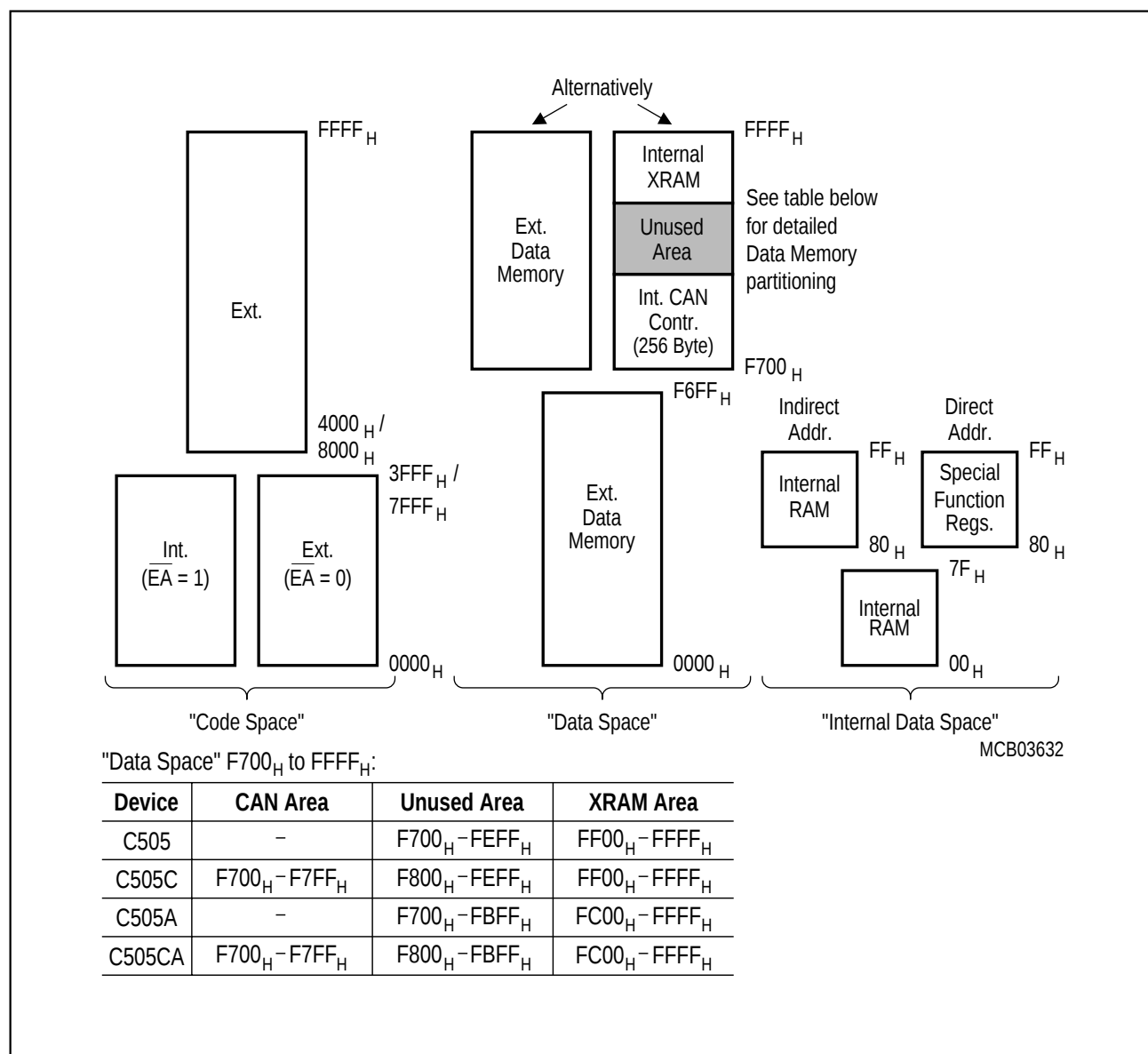
Figure 5 C505 Memory Map
