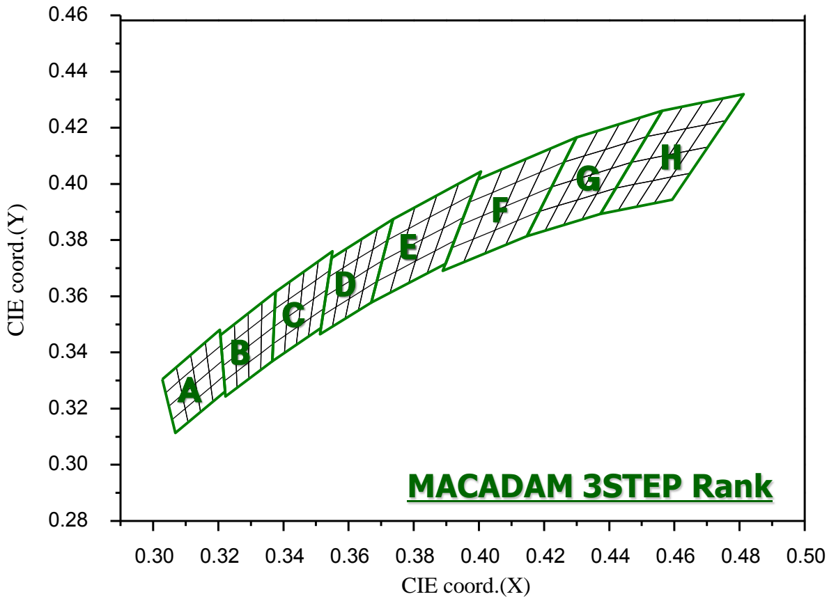
CIE Chromaticity Diagram, T_j = 25^\circ\text{C} , I_F = 100\text{mA}
