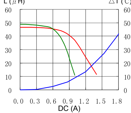
17. CDRH6D38NP-820NC
