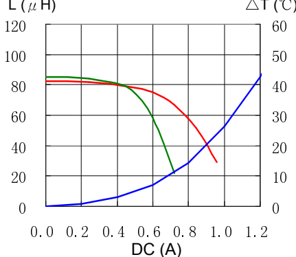
17. CDRH6D38NP-820NC
