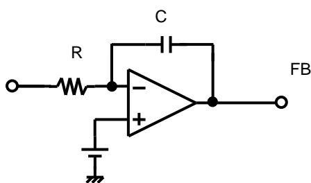
Figure 41. General Integrator
