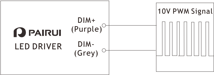
PWM Dimming
