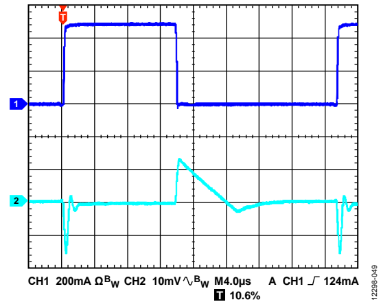
Figure 49. Load Transient Response, I_{LOAD} = 10\text{ mA} to 500\text{ mA} , V_{OUT} = 5\text{ V} , V_{IN} = 5.5\text{ V} , CH1 = I_{LOAD} , CH2 = V_{OUT}
