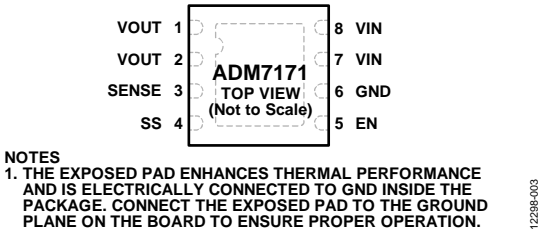
Figure 3. Pin Configuration
