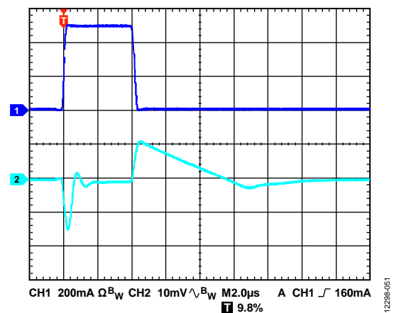
Figure 51. Load Transient Response, I_{LOAD} = 10\text{ mA} to 500\text{ mA} , Adjustable Version, V_{OUT} = 1.2\text{ V} , V_{IN} = 2.5\text{ V} , CH1 = I_{LOAD} , CH2 = V_{OUT}
