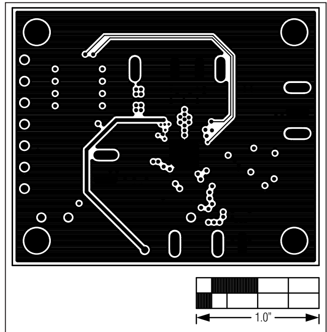
Figure 5. MAX17019N EV Kit PCB Layout—Layer 3
