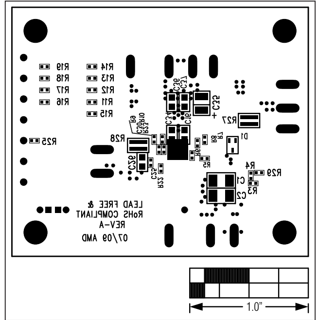
Figure 7. MAX17019N EV Kit Component Placement Guide—Solder Side
