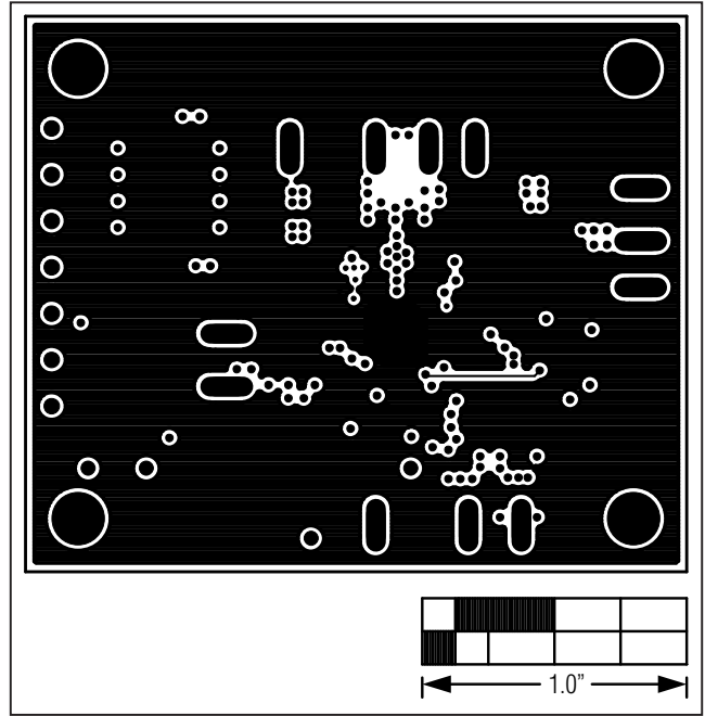
Figure 4. MAX17019N EV Kit PCB Layout—Layer 2
