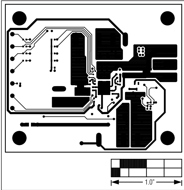
Figure 6. MAX17019N EV Kit PCB Layout—Solder Side
