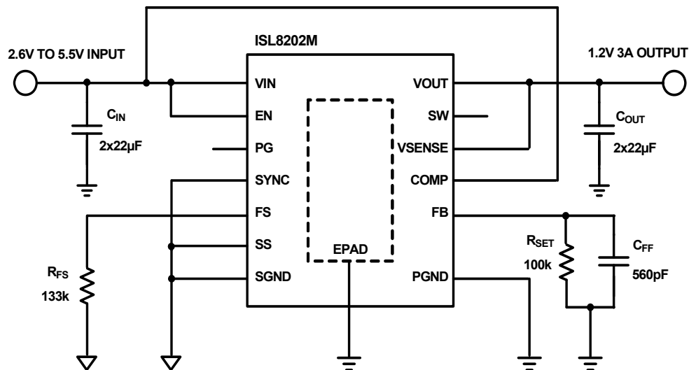
FIGURE 38. TYPICAL APPLICATION CIRCUIT DIAGRAM IN PFM MODE
