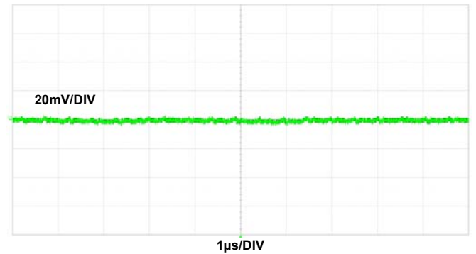
FIGURE 13. V_{IN} = 3.3V , V_{OUT} = 2.5V , I_{OUT} = 3A , f_{SW} = 2MHz , C_{OUT} = 2 \times 22\mu F CERAMIC CAPACITORS
