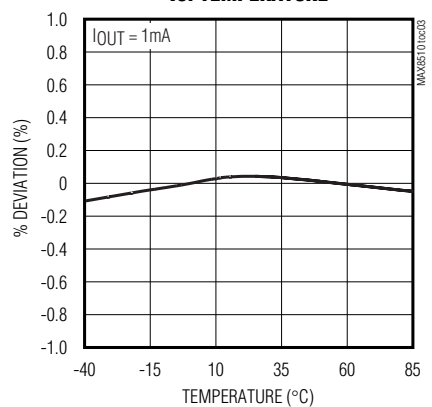
MAX8510 OUTPUT VOLTAGE ACCURACY vs. TEMPERATURE
