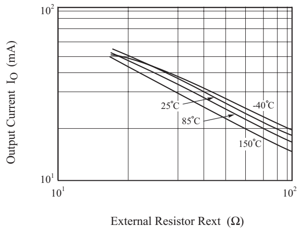
I_O - R_{ext}
