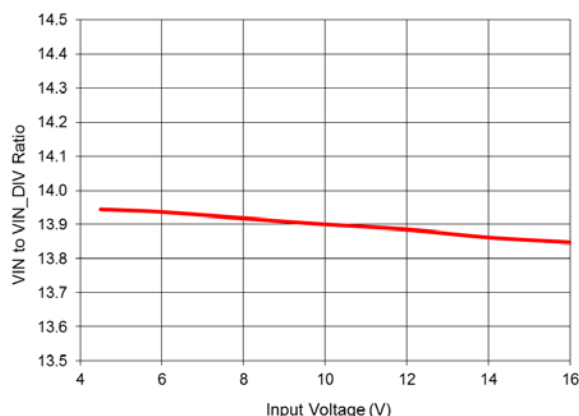
Figure 30: VIN to VIN_DIV Ratio
