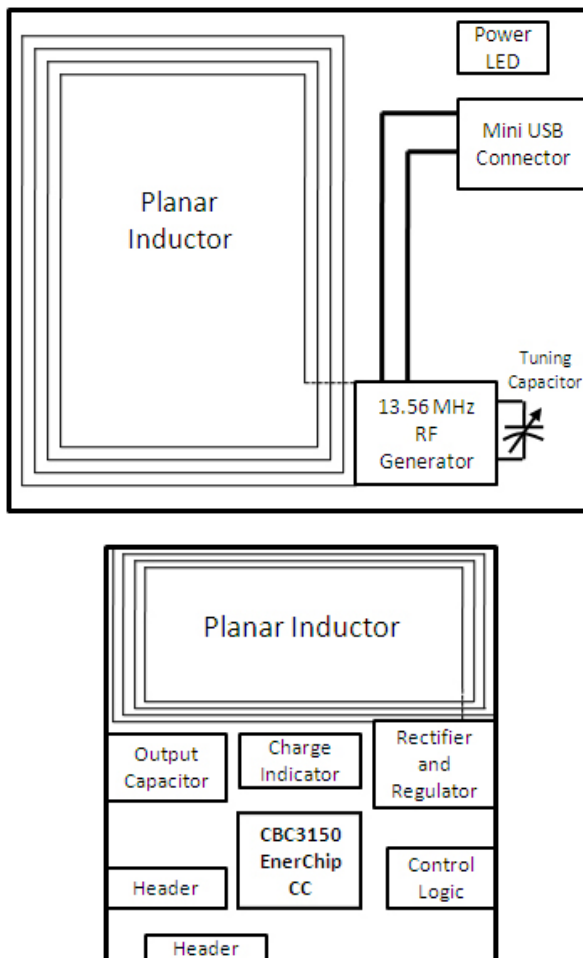
Figure 1: Block Diagram of CBC-EVAL-11 Evaluation Kit - transmitter board (top) and receiver board (bottom).
