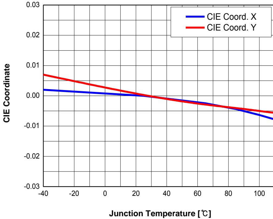
Fig 8. Chromaticity Coordinate vs. Junction Temperature, I_F = 10\text{mA}
