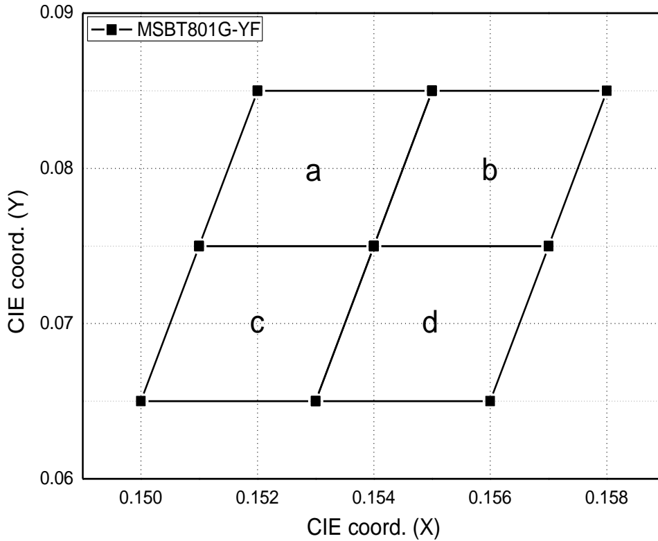
CIE Chromaticity Diagram, I_F = 10\text{mA} , T_j = 25^\circ\text{C}
