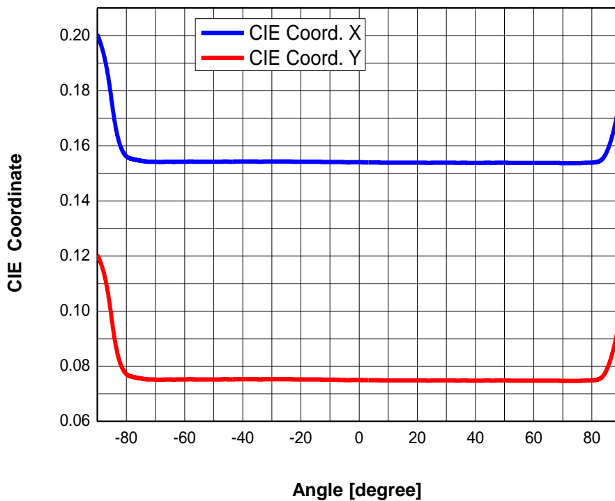
Fig 10. Color. vs. Viewing Angle, T_j = 25^\circ\text{C} , I_F = 10\text{mA}
