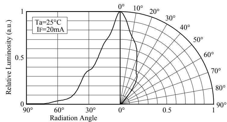
■ Directivity (NSPB520S)
