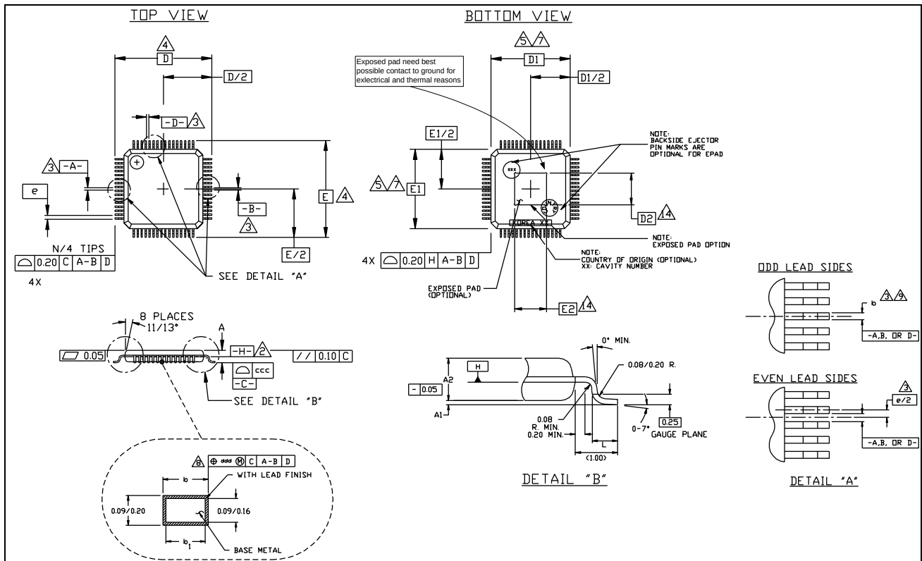
Figure 6 – TQFP 7x7 Drawing
