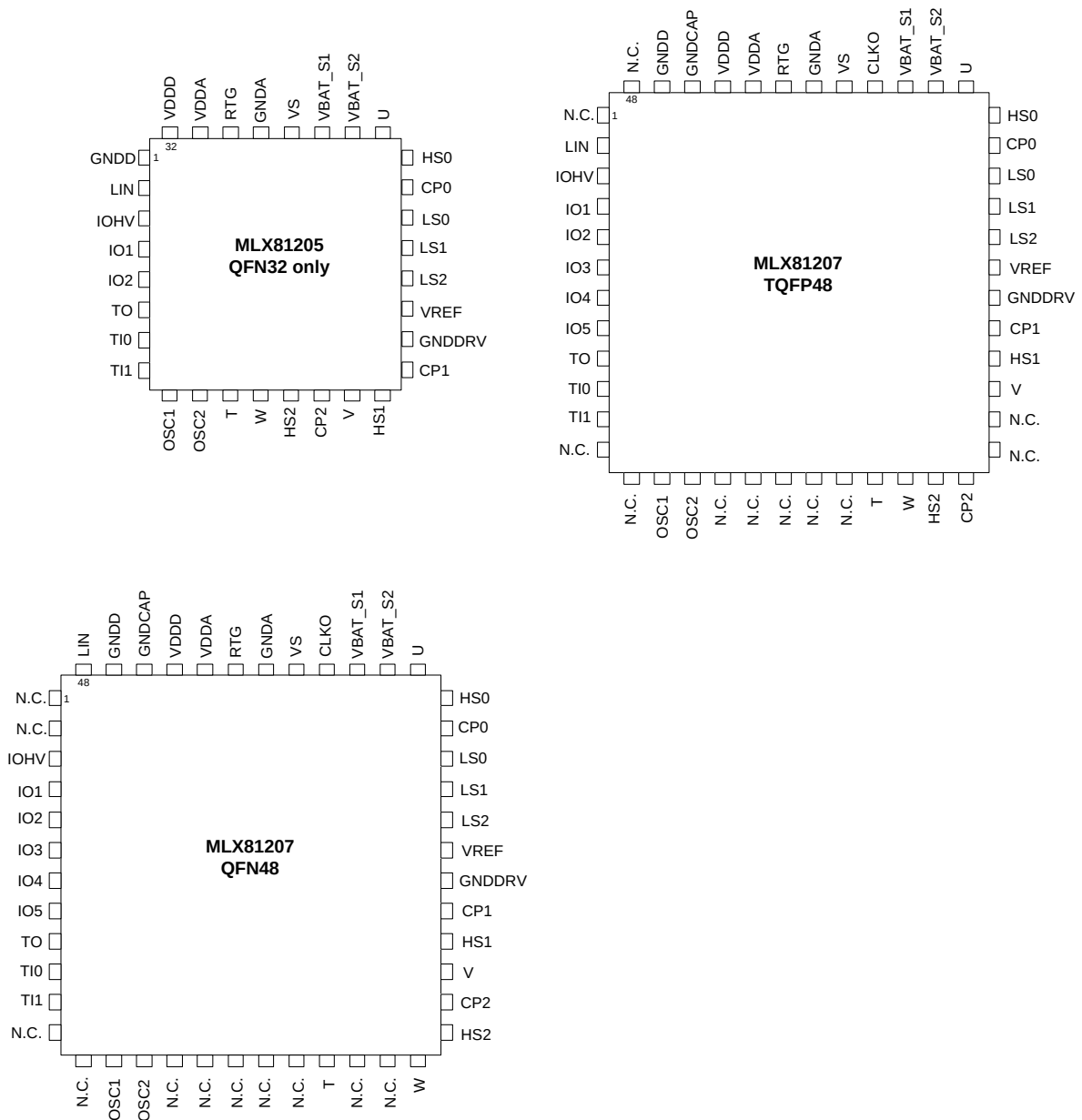
Figure 8 – MLX81205/07 Pins
