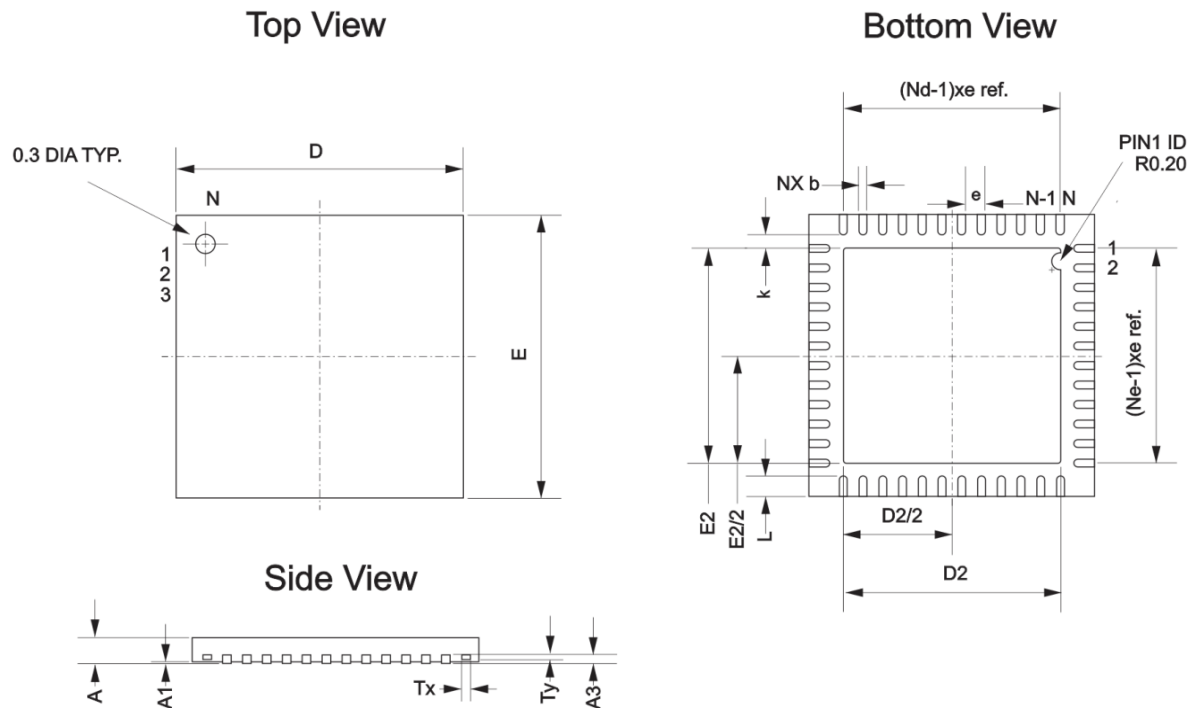
Figure 5 - QFN Package Drawing
