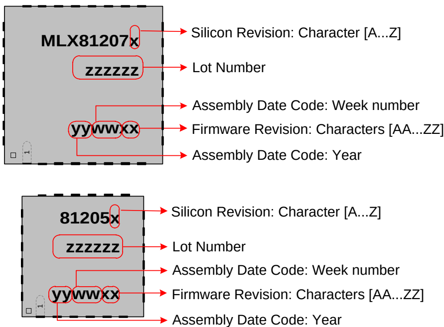
Figure 7 – Marking Code
