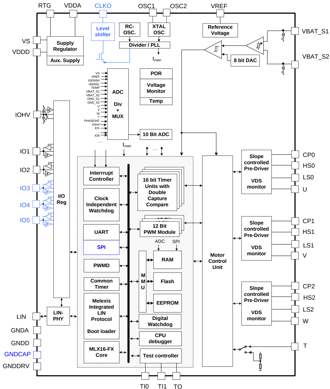
Figure 1 – Block Diagram
