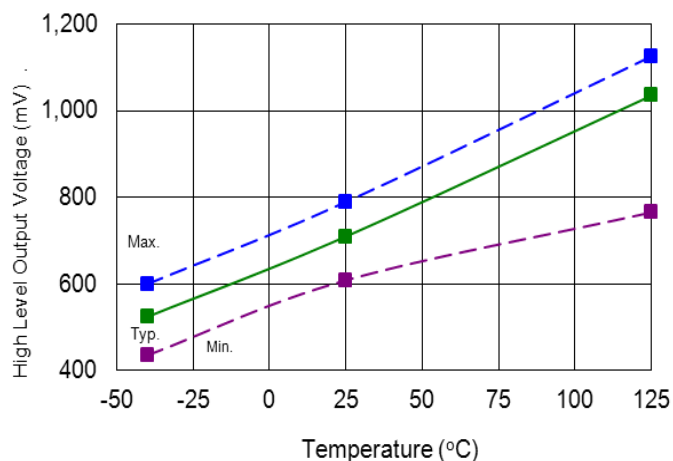
Figure 36. High Level Output Voltage vs. Temperature I_o = 20\text{mA}
