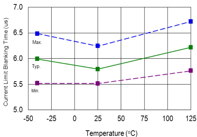
Figure 19. Current Limit Blanking Time vs. Temperature
