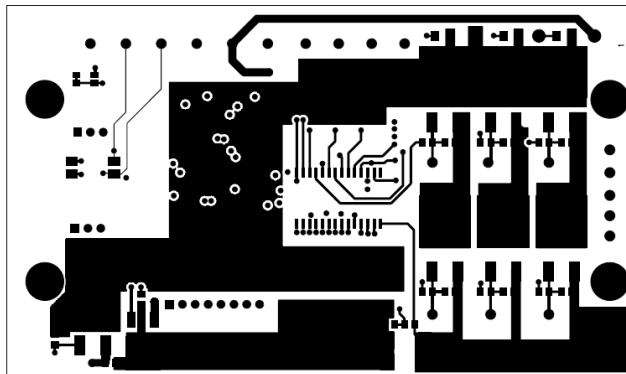
Figure 10: Component Face Layout
