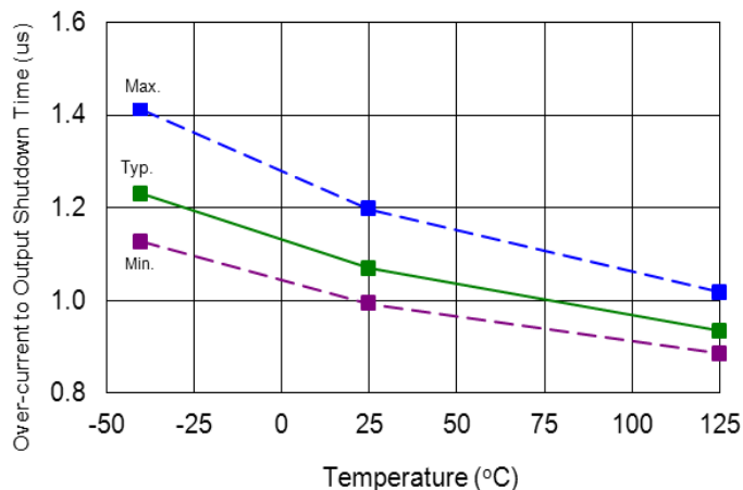
Figure 21. Over Current Shutdown Time vs. Temperature
