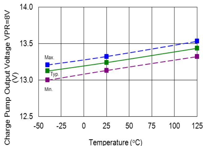
Figure 40. Charge Pump Output Voltage vs. Temperature VPR = 8\text{V}
