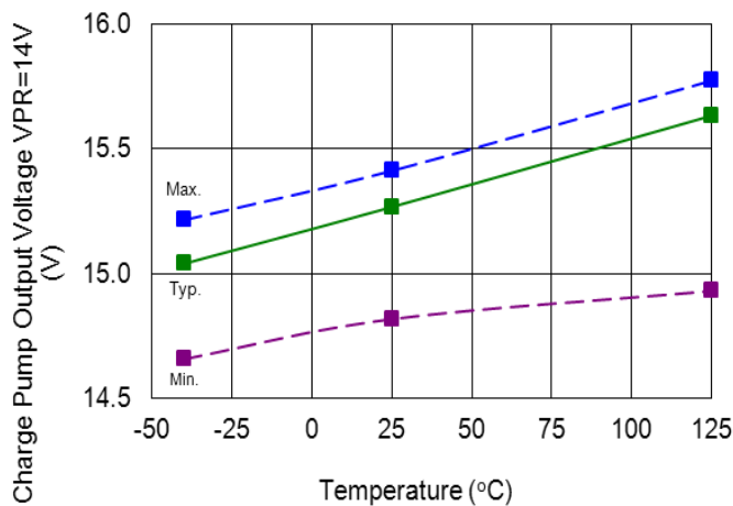
Figure 41. Charge Pump Output Voltage vs. Temperature VPR = 14\text{V}
