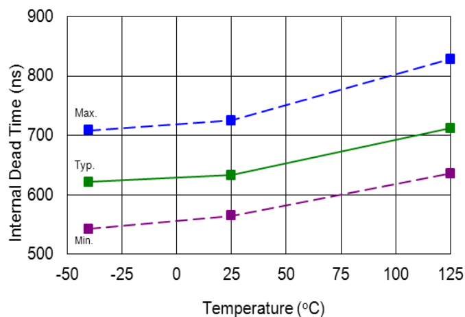
Figure 22. Dead Time vs. Temperature
