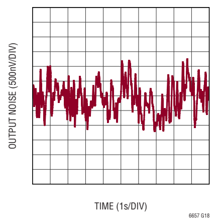
5V Low Frequency 0.1Hz to 10Hz Noise
