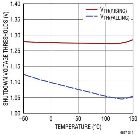
Shutdown Voltage Thresholds vs Temperature
