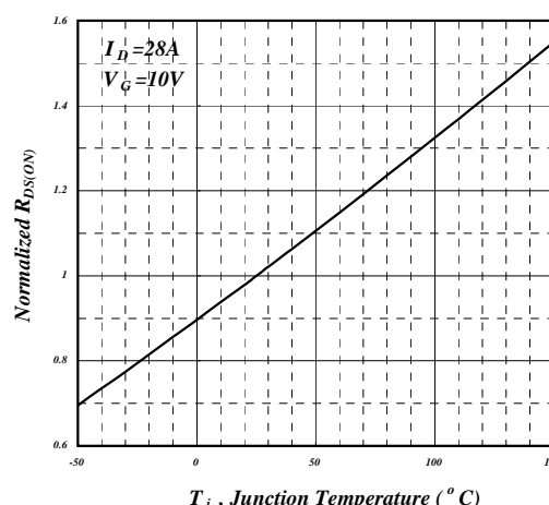
Fig 4. Normalized On-Resistance
