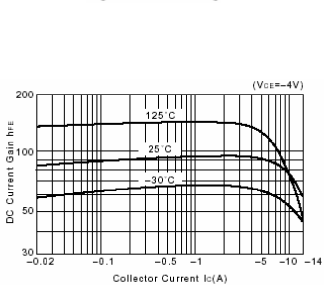
Fig.8 DC current Gain
