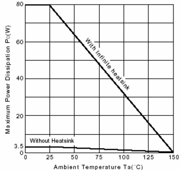
Fig.6 P_c-T_a Derating
