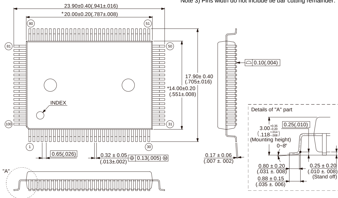
Note 1) * : These dimensions do not include resin protrusion. Note 2) Pins width and pins thickness include plating thickness. Note 3) Pins width do not include tie bar cutting remainder.
