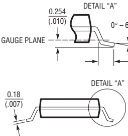
RECOMMENDED SOLDER PAD LAYOUT
