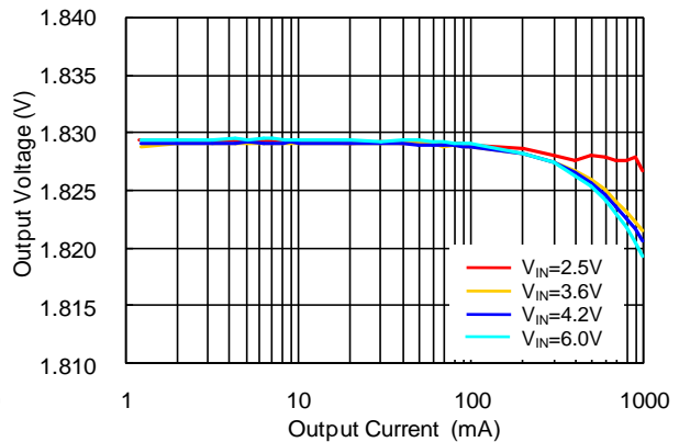
Output Voltage vs. Load Current V OUT =1.8V, MODE=H
