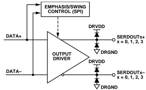
Figure 107. Digital Outputs
