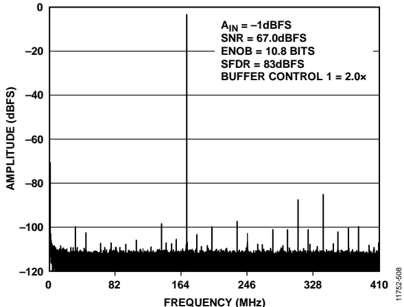
Figure 56. Single-Tone FFT with f_{IN} = 170.3 MHz
