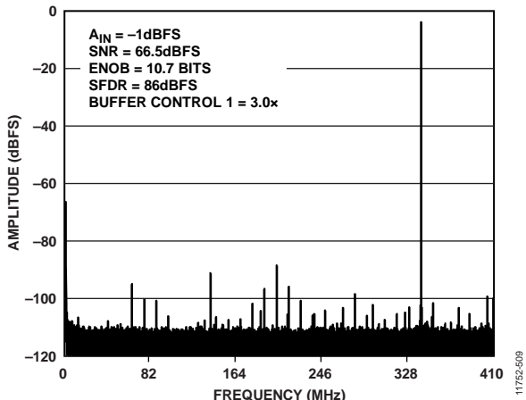
Figure 57. Single-Tone FFT with f_{IN} = 340.3 MHz
