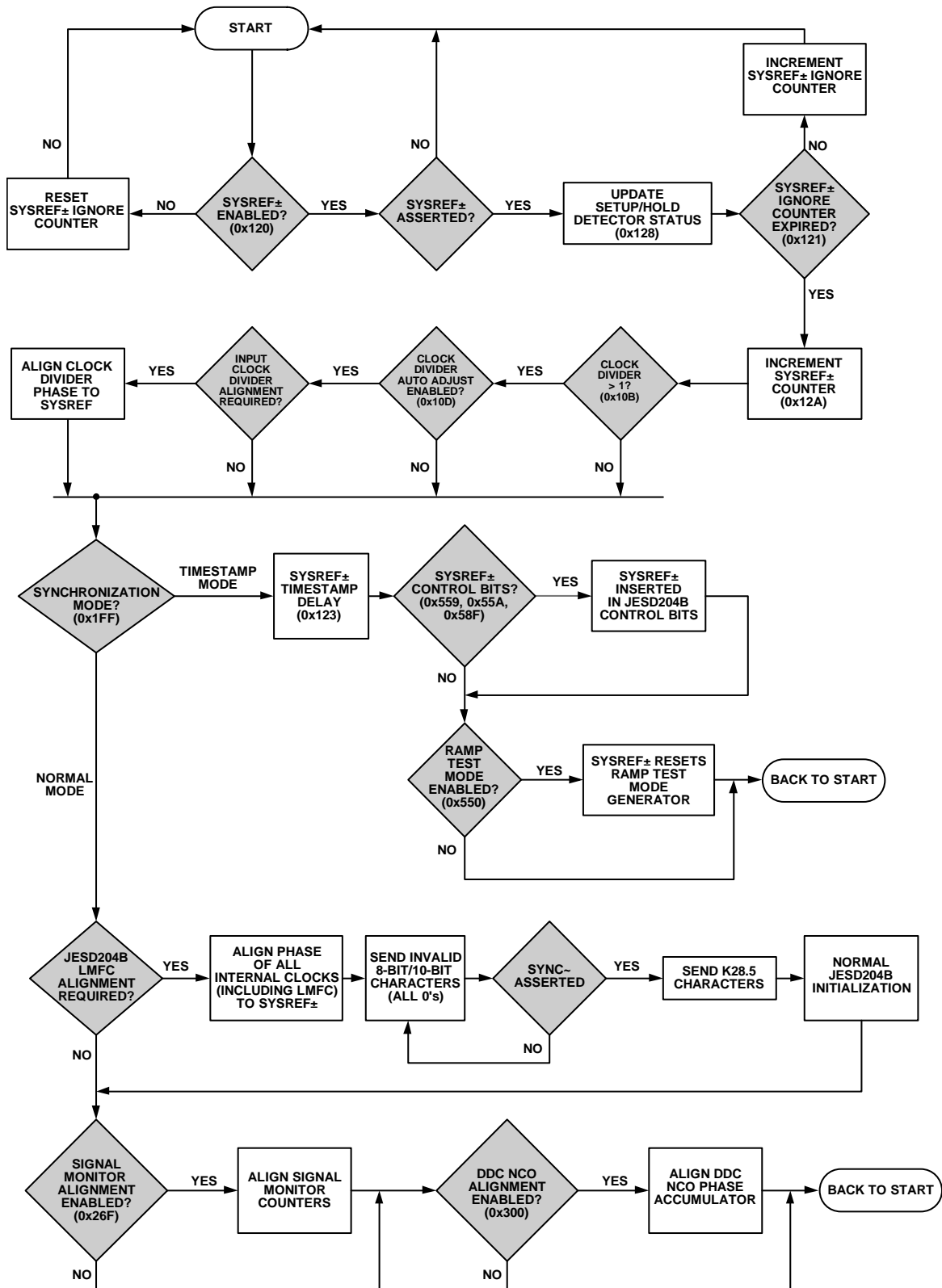
Figure 171. Multichip Synchronization
