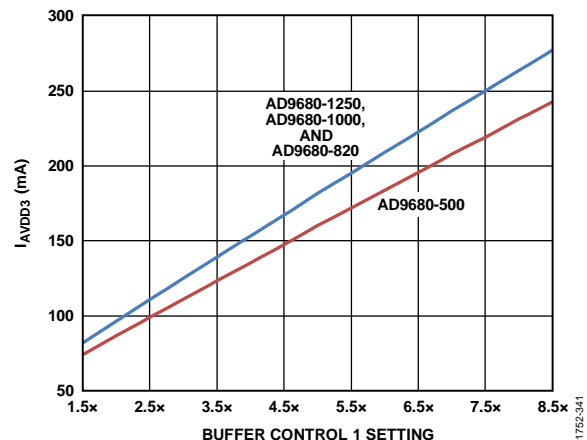
Figure 117. I AVDD3 vs. Buffer Control 1 Setting in Register 0x018
