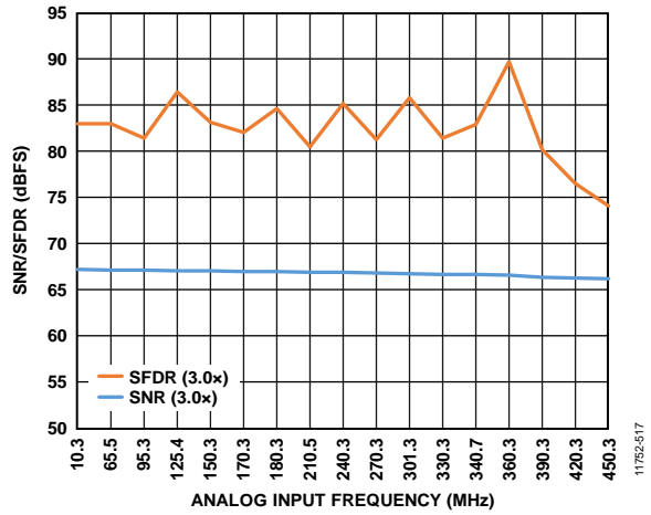
Figure 65. SNR/SFDR vs. f_{IN} ; f_{IN} < 450 MHz; Buffer Control 1 (0x018) = 3.0x
