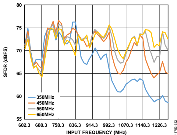
Figure 119. Buffer Current Sweeps, AD9680-1250 (SFDR vs. I_{BUFF} ); 600 MHz < f_{IN} < 1300 MHz; Front-End Network Shown in Figure 115
