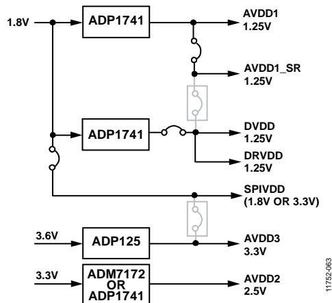
Figure 174. High Efficiency, Low Noise Power Solution for the AD9680
