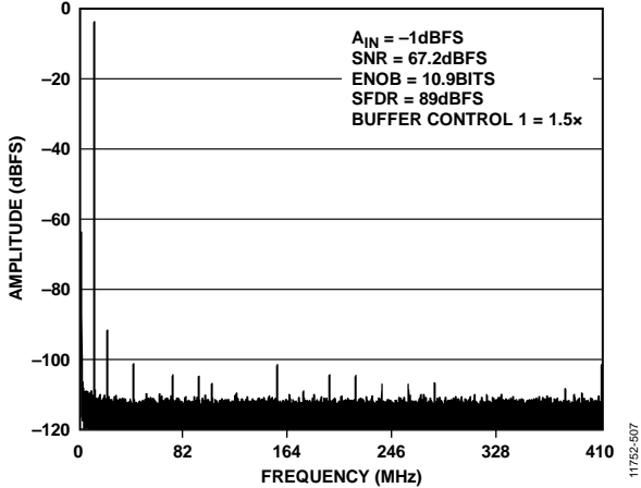
Figure 55. Single-Tone FFT with f_{IN} = 10.3 MHz
