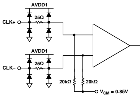
Figure 105. Clock Inputs
