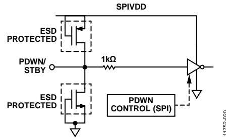
Figure 113. PDWN/STBY Input
