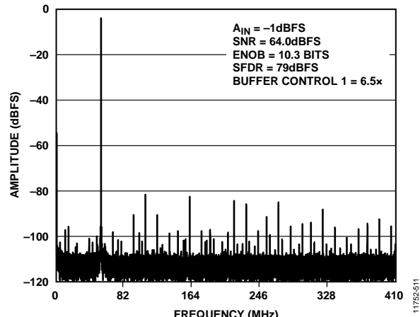
Figure 59. Single-Tone FFT with f_{IN} = 765.3 MHz
