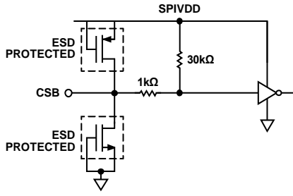
Figure 110. CSB Input
