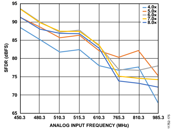
Figure 129. Buffer Current Sweeps, AD9680-500 (SFDR vs. I_{BUFF} ); 450 \text{ MHz} < f_{IN} < 1000 MHz; Front-End Network Shown in Figure 115
