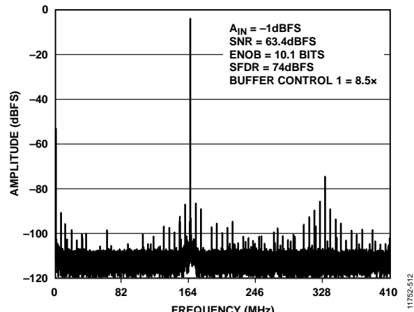
Figure 60. Single-Tone FFT with f_{IN} = 985.3 MHz
