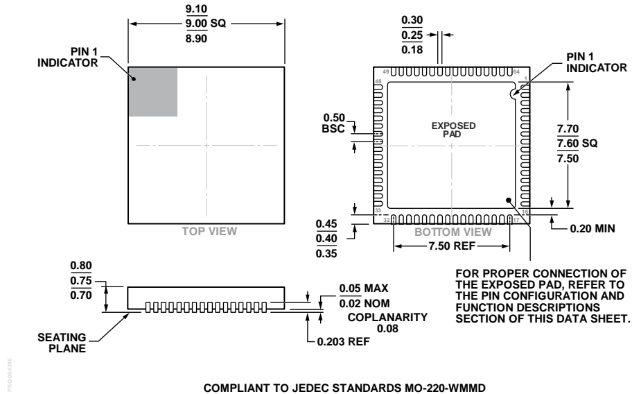
Figure 176. 64-Lead Lead Frame Chip Scale Package [LFCSP_WQ] 9 mm × 9 mm Body, Very Thin Quad (CP-64-15) Dimensions shown in millimeters
