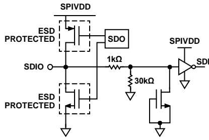
Figure 111. SDIO Input
