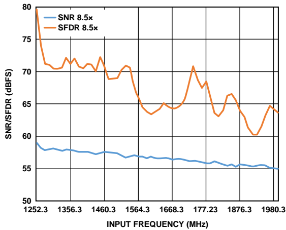
Figure 18. SNR/SFDR vs. f_{IN} ; 1.3 \text{ GHz} < f_{IN} < 2 \text{ GHz} ; Buffer Control 1 (0x018) = 8.5x
