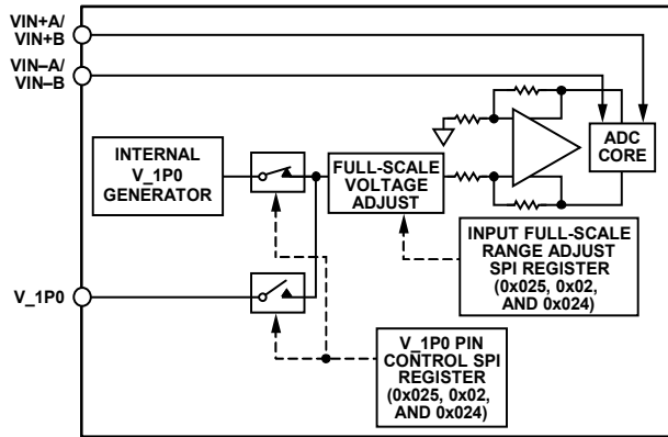
Figure 131. Internal Reference Configuration and Controls
