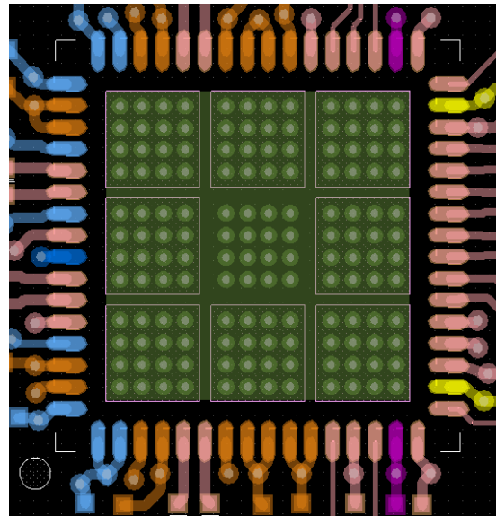
Figure 175. Recommended PCB Layout of Exposed Pad for the AD9680
