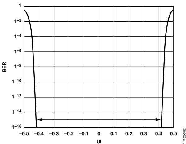
Figure 163. Digital Outputs Bathtub Curve, External 100 Ω Terminations at 10 Gbps
