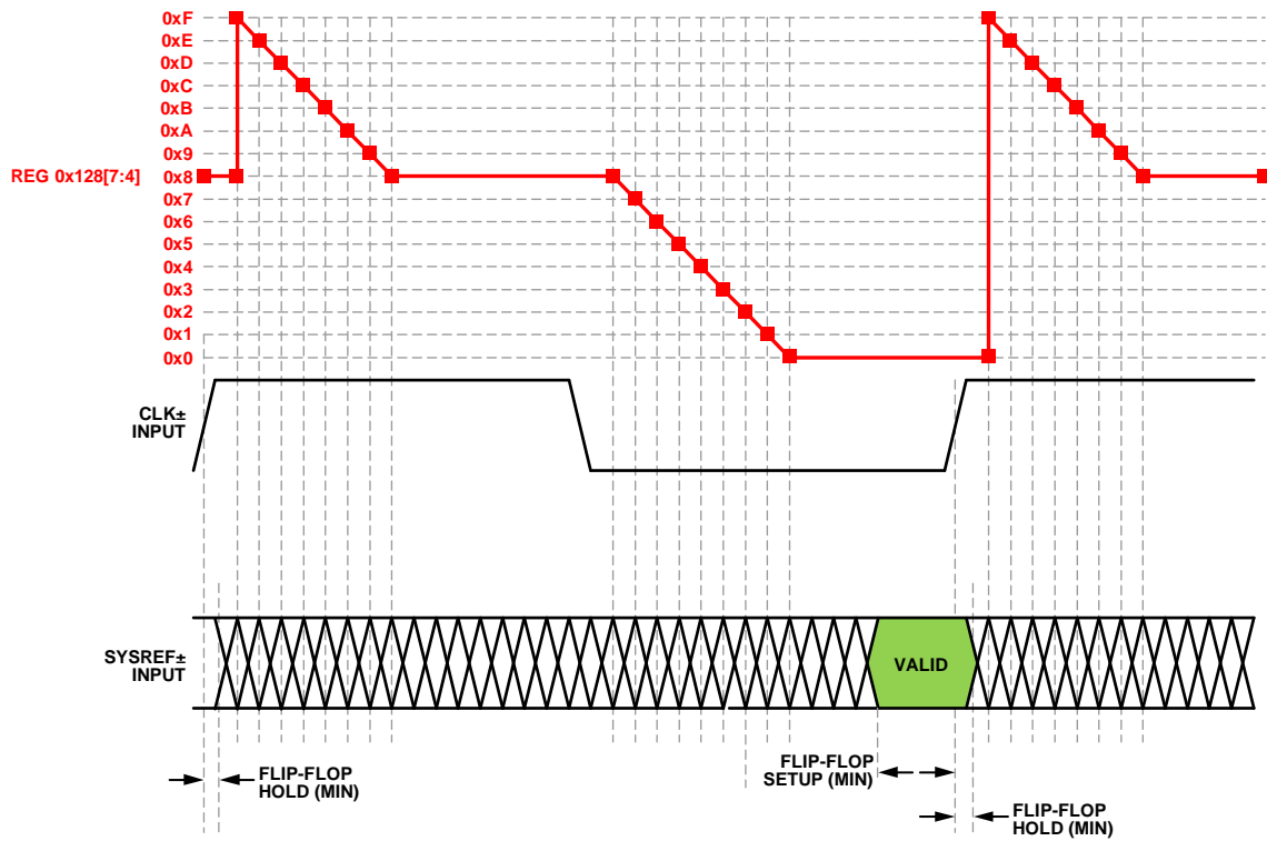
Figure 173. SYSREF± Hold Detector
