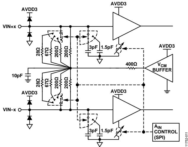
Figure 104. Analog Inputs
