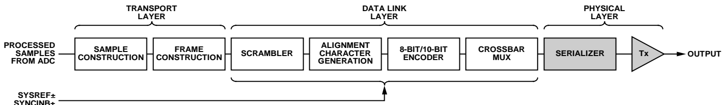
Figure 157. Data Flow
