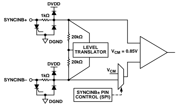
Figure 108. SYNCINB± Inputs
