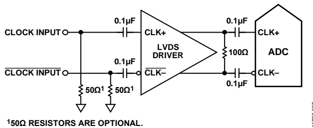
Figure 136. Differential LVDS Sample Clock
