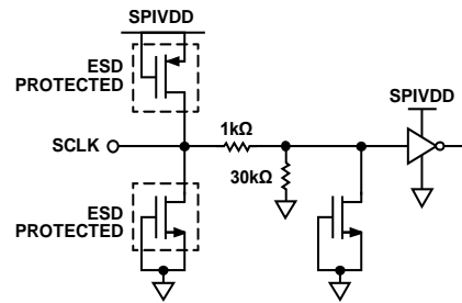
Figure 109. SCLK Input
