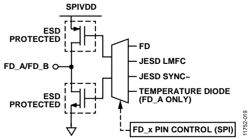
Figure 112. FD_A/FD_B Outputs
