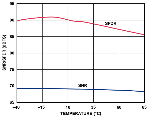
Figure 98. SNR/SFDR vs. Temperature, f_{IN} = 170.3 MHz
