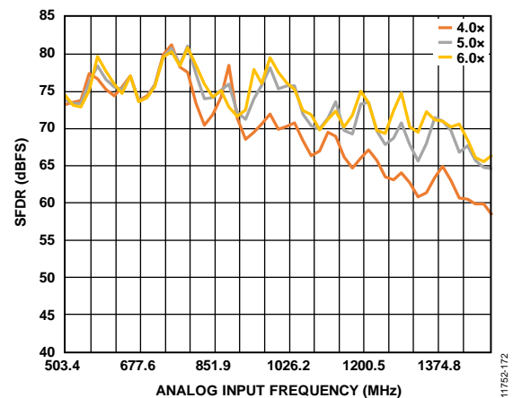
Figure 122. Buffer Current Sweeps, AD9680-1000 (SFDR vs. I_{BUFF} ); 500 MHz < f_{IN} < 1500 MHz; Front-End Network Shown in Figure 115
