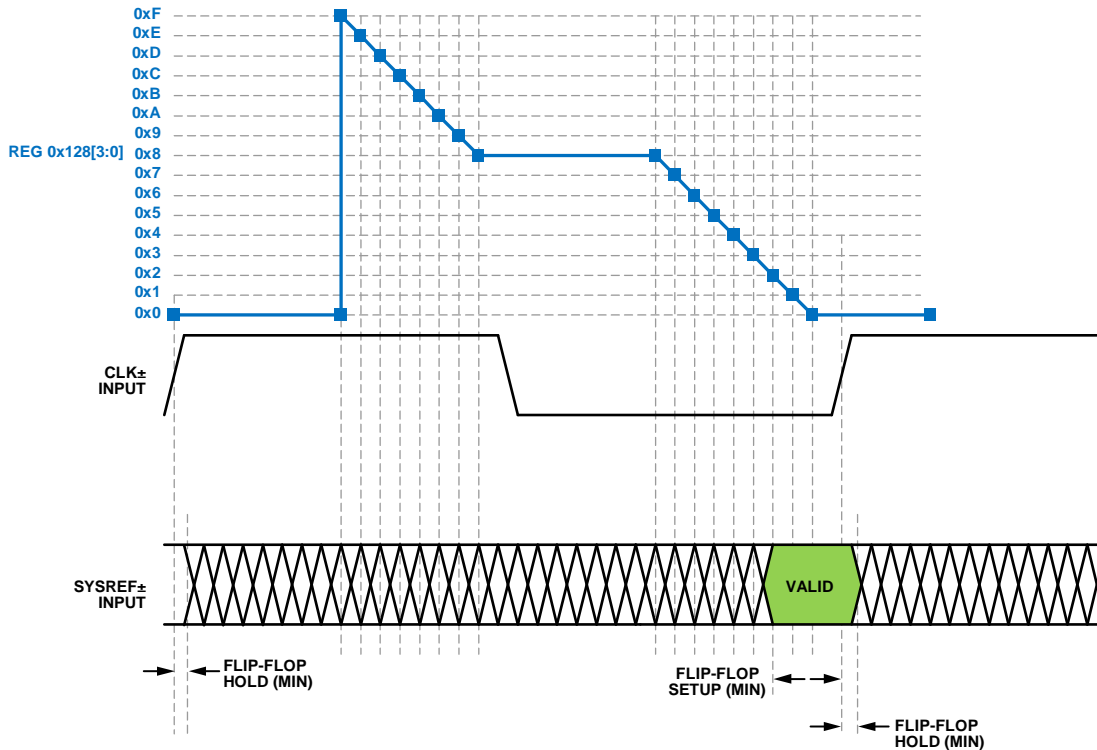
Figure 172. SYSREF± Setup Detector
