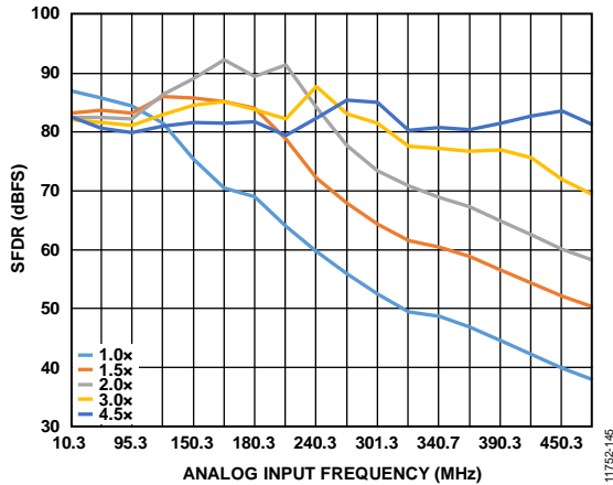
Figure 128. Buffer Current Sweeps, AD9680-500 (SFDR vs. I_{BUFF} ); f_{IN} < 500 MHz; Front-End Network Shown in Figure 115 Buffer Control 1 (0x018) = 1.0x, 1.5x, 2.0x, 3.0x, or 4.5x
