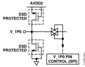
Figure 114. V_1P0 Input/Output
