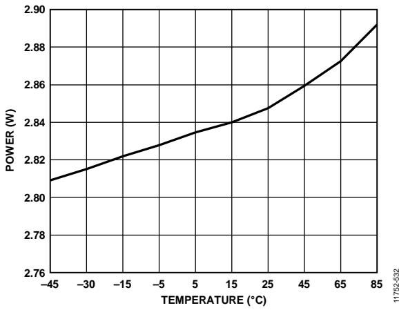
Figure 78. Power Dissipation vs. Temperature
